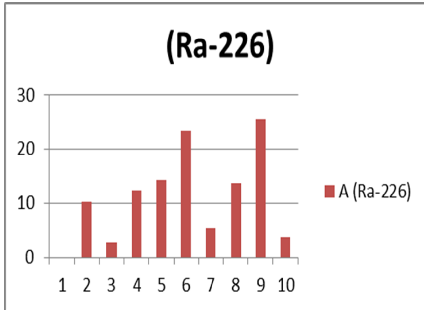
Fig1: 226 Ra isotopes concentration in biscuit samples under study.
