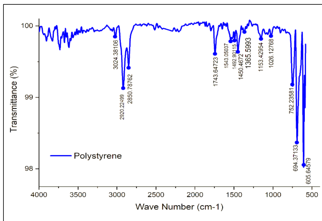
(Fig.4). Infrared spectrum of the polystyrene
